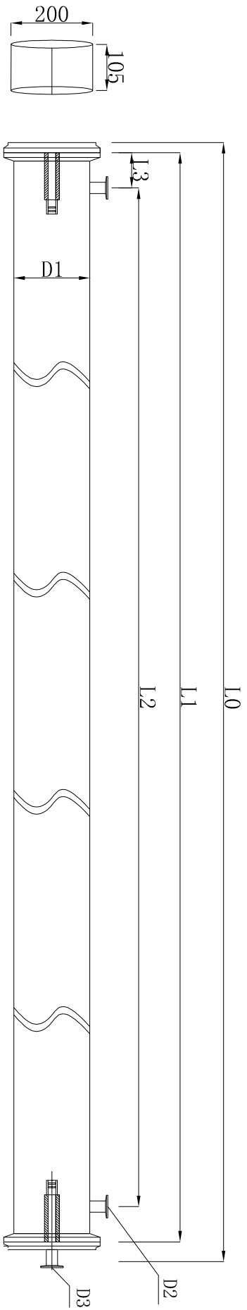
8英寸5芯膜壳图纸
